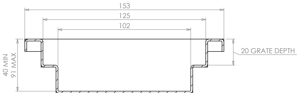
SECTION VIEW
